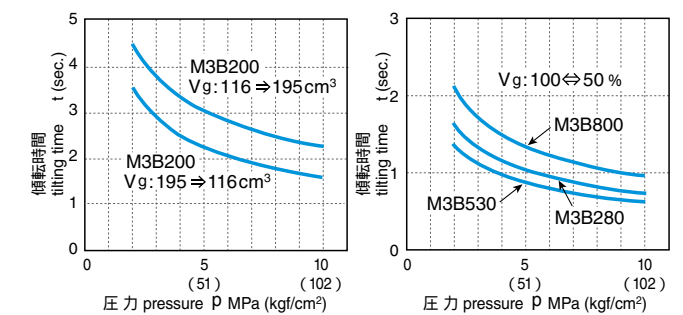
圧力と傾転時間 / Tilting time, pressure related
