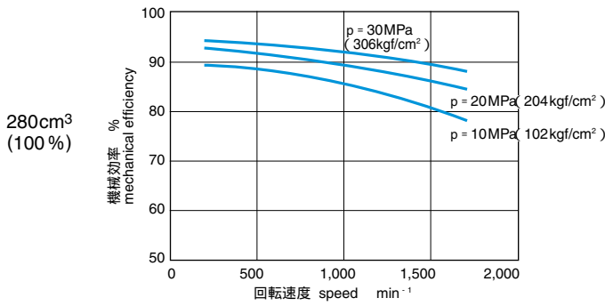
機械効率 / Mechanical efficiency (%)
