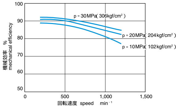
機械効率 / Mechanical efficiency (%)
